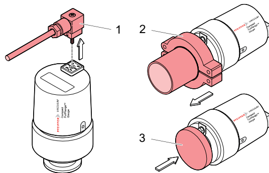
Fig. 8: Removing gauge
