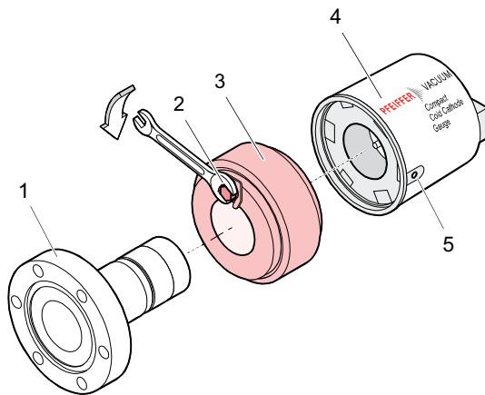
Fig. 3: Removing/installing magnetic unit
