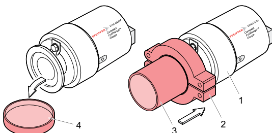
Fig. 2: Establishing vacuum connection
