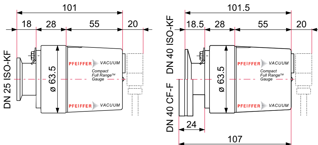
Fig. 12: Dimensions Dimensions in mm
