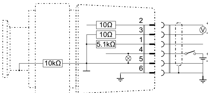
Fig. 4: Connection diagram
