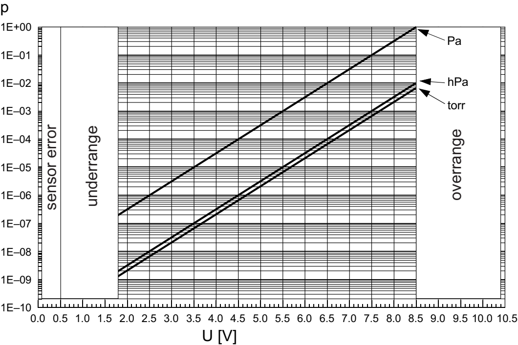
Fig. 6: Relation between measuring signal and pressure
