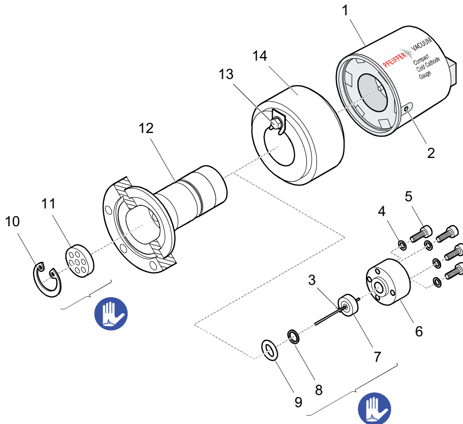
Fig. 9: Individual parts
