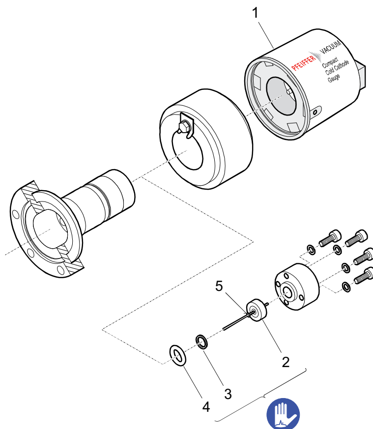
Fig. 11: Spare parts
