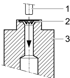
Fig. 10: Mounting tool for the ignition aid
